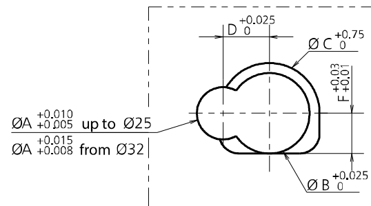
POCKET DIMENSIONS
